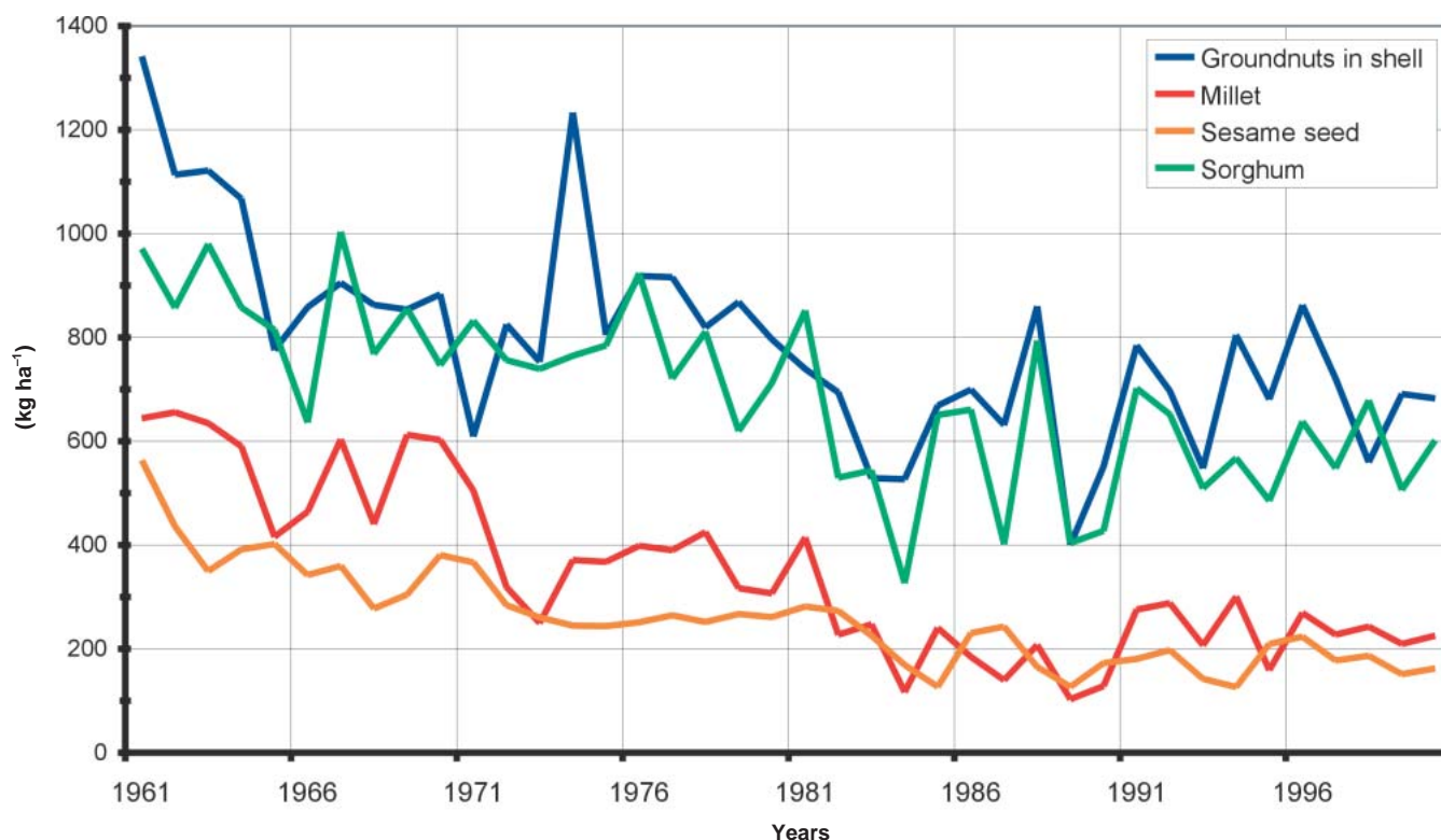
Figure 6. Yield of groundnuts, millet, sesame and sorghum from The Sudan, 1961–2000. Source of data: FAO.
