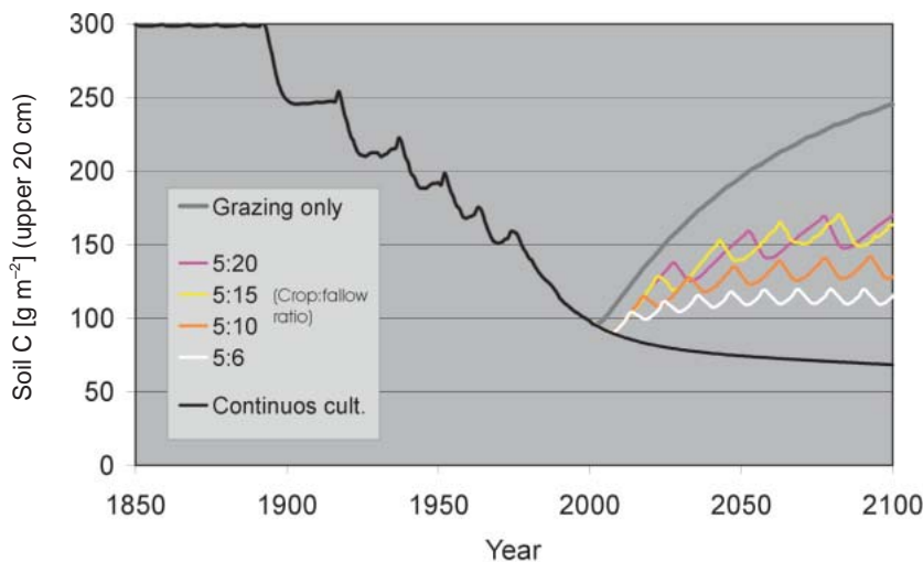
Figure 5. Recovery scenarios for site B, based on modelling of soil organic carbon content according to the scenarios described in the text.
