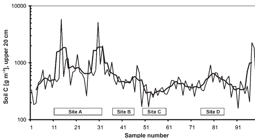
Figure 2. Soil organic carbon content (0–20 cm, \text{g m}^{-2} ) measured in 1980 along the transect shown in Figure 1. Numbers on the x-axis refer to sampling numbers in Figure 1. Note the logarithmic scale. The solid line is a 5 sample running mean.
