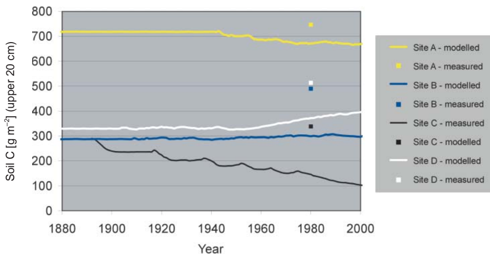
Figure 4. Result of the modelling of soil organic carbon content (lines) and the measured values (symbols).
