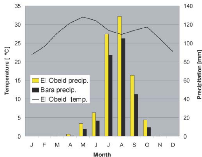
Figure 3. Mean monthly temperature for El Obeid and mean precipitation for El Obeid and Bara.
